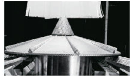
Adjustable rotating topcone
